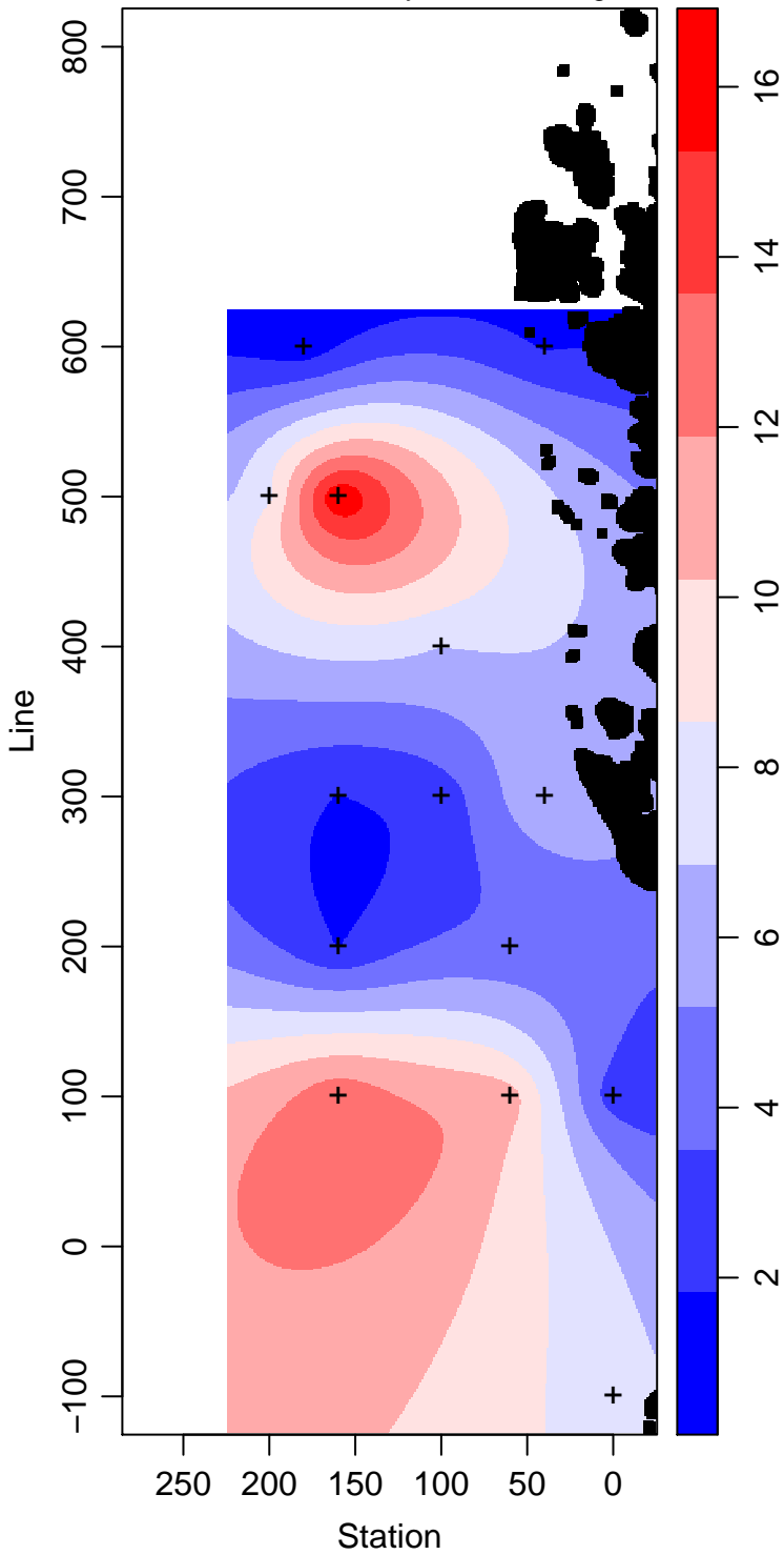
LMG09-01_45_Primary.Production mg m -3
