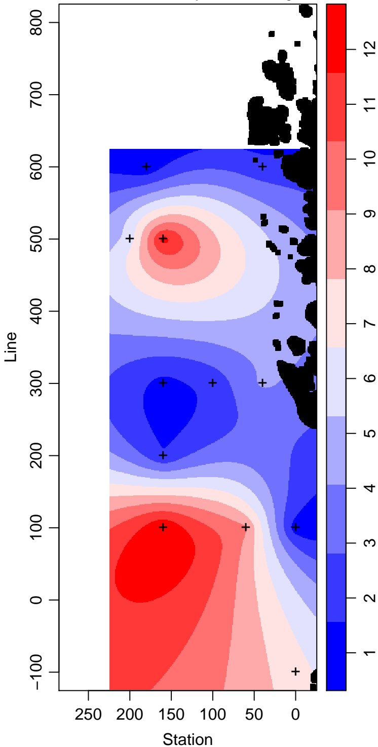
LMG09-01_50_Primary.Production mg m -3
