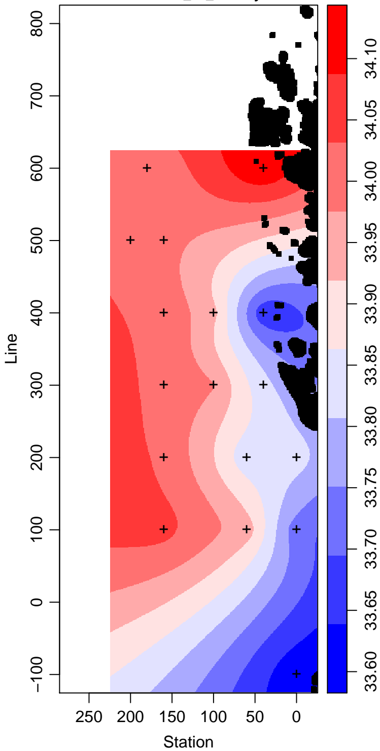
LMG09-01_45_Salinity
