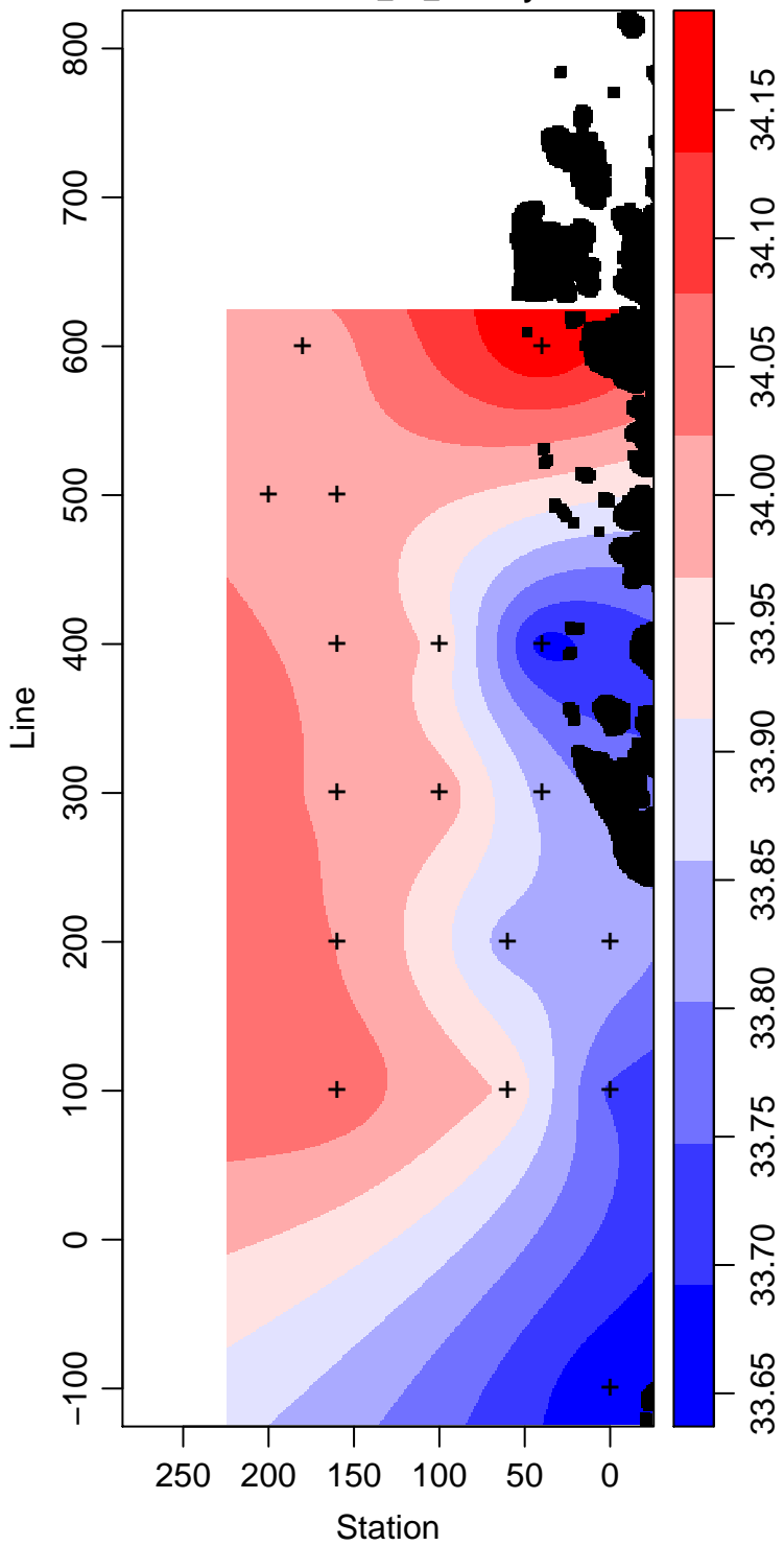
LMG09-01_50_Salinity
