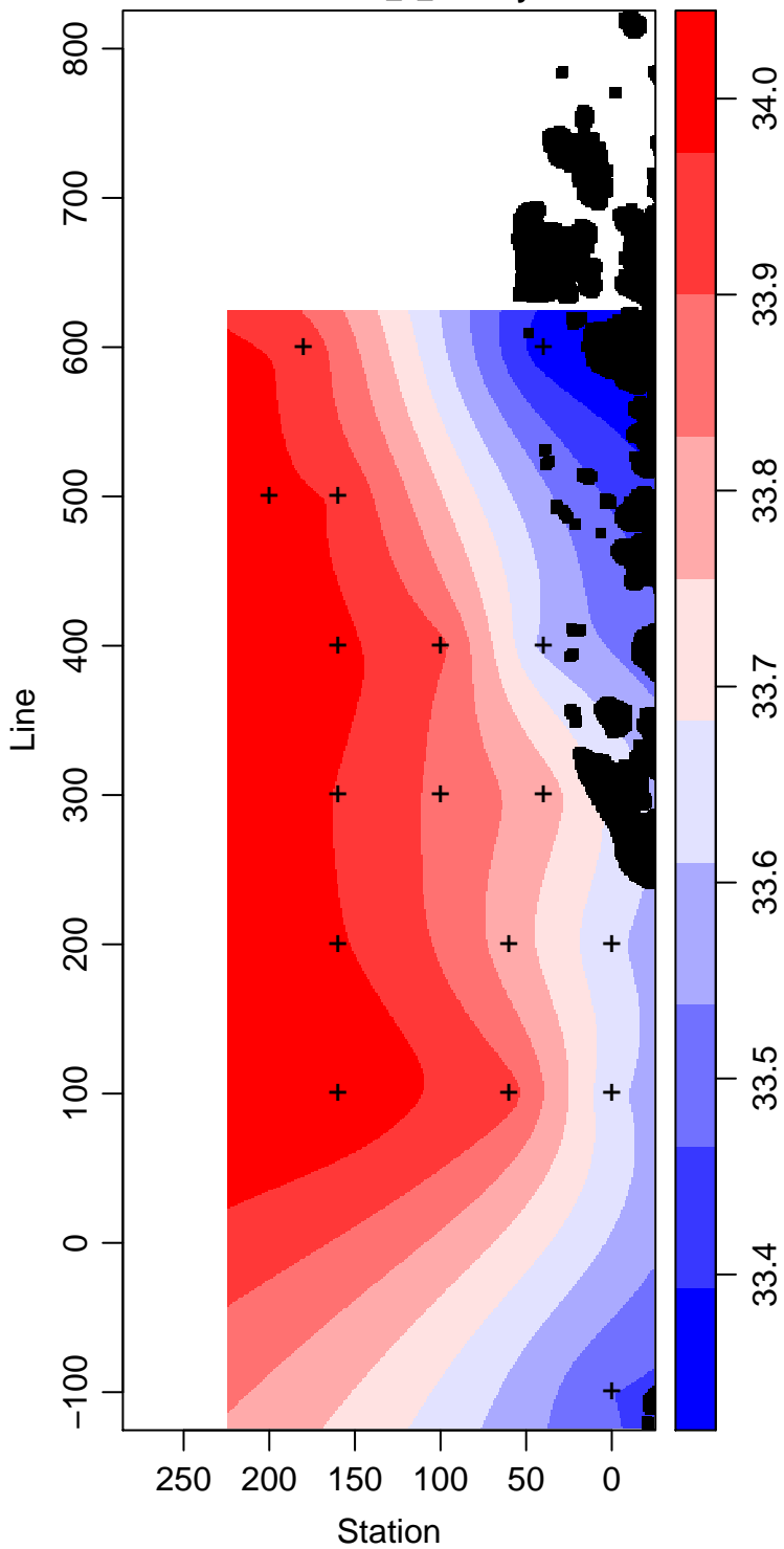
LMG09-01_5_Salinity
