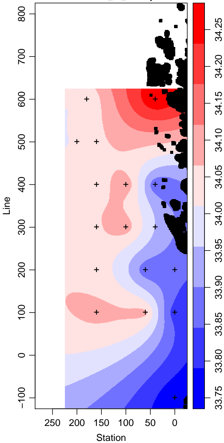
LMG09-01_65_Salinity
