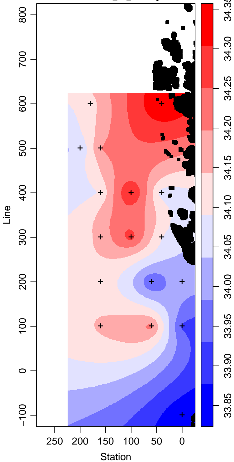
LMG09-01_85_Salinity
