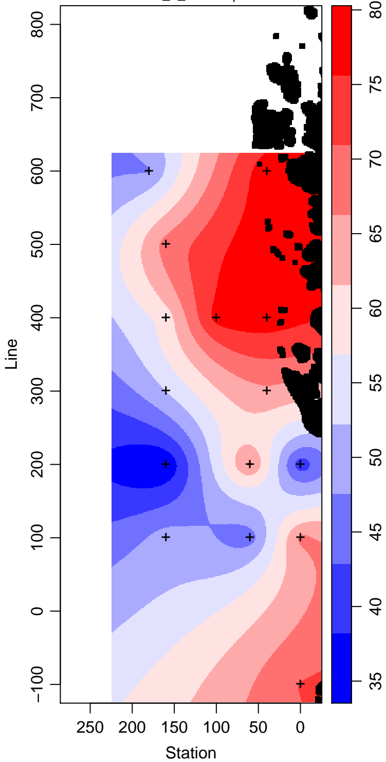
LMG09-01_1_Silicate \mu\text{ mol L}^{-1}
