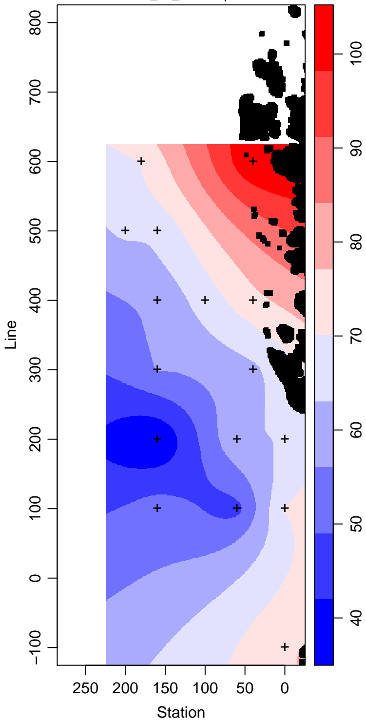
LMG09-01_45_Silicate \mu\text{ mol L}^{-1}
