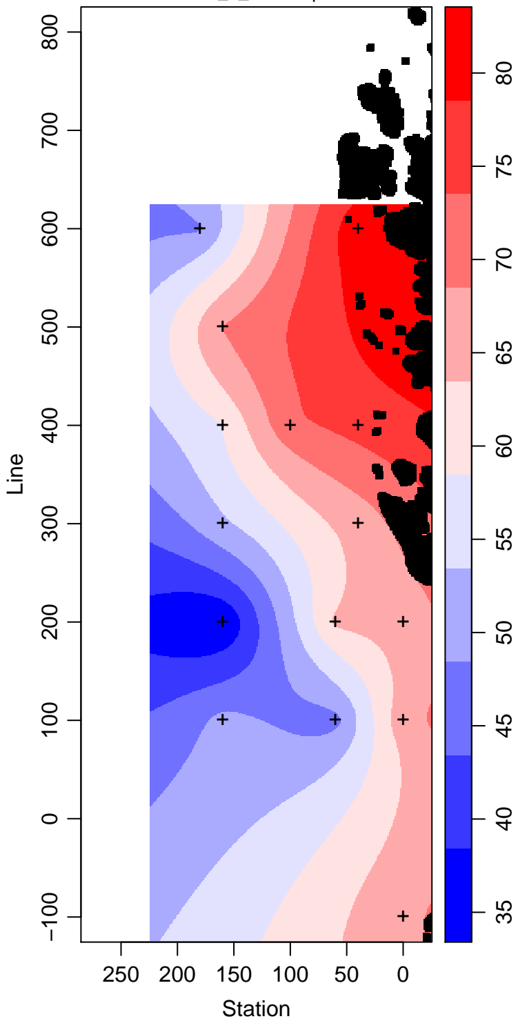
LMG09-01_5_Silicate \mu\text{ mol L}^{-1}
