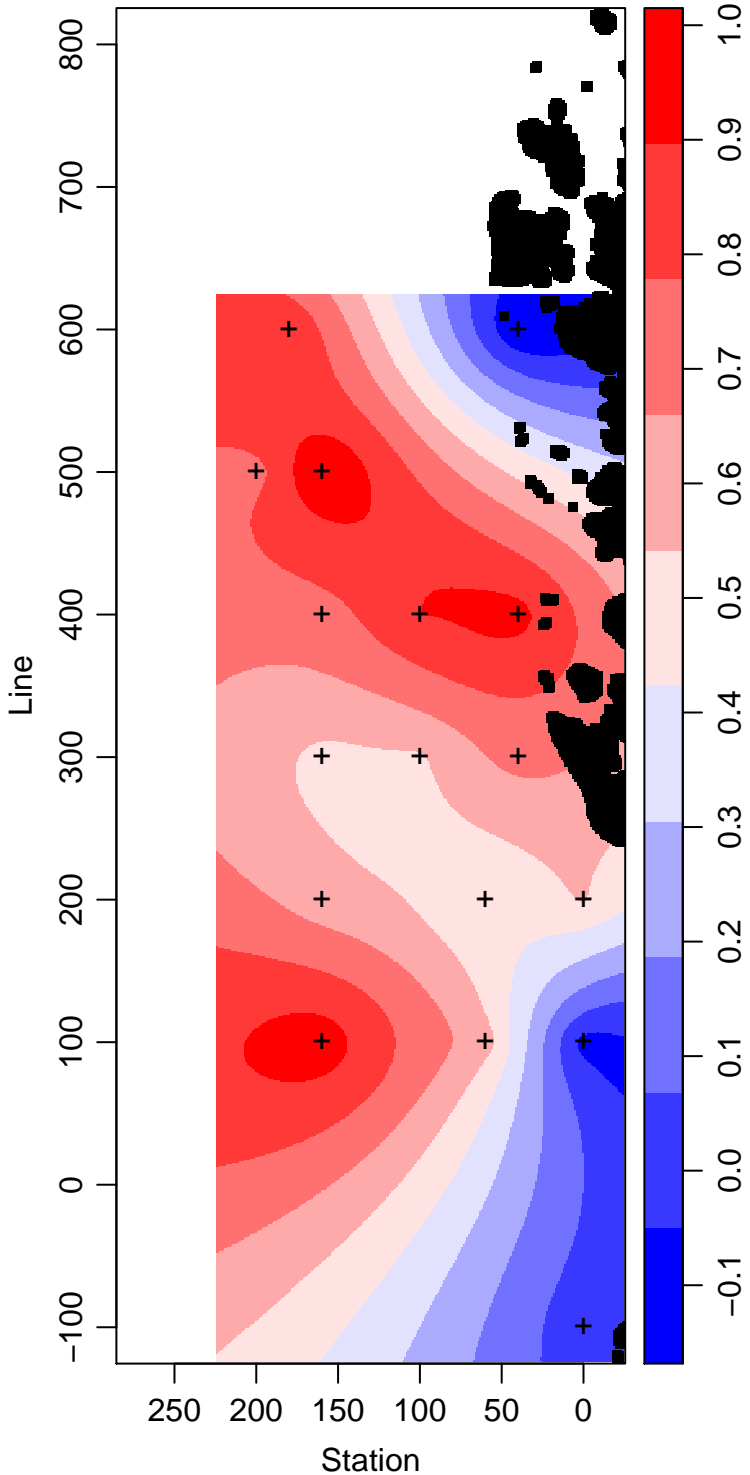
LMG09-01_25_Temperature ° Celsius
