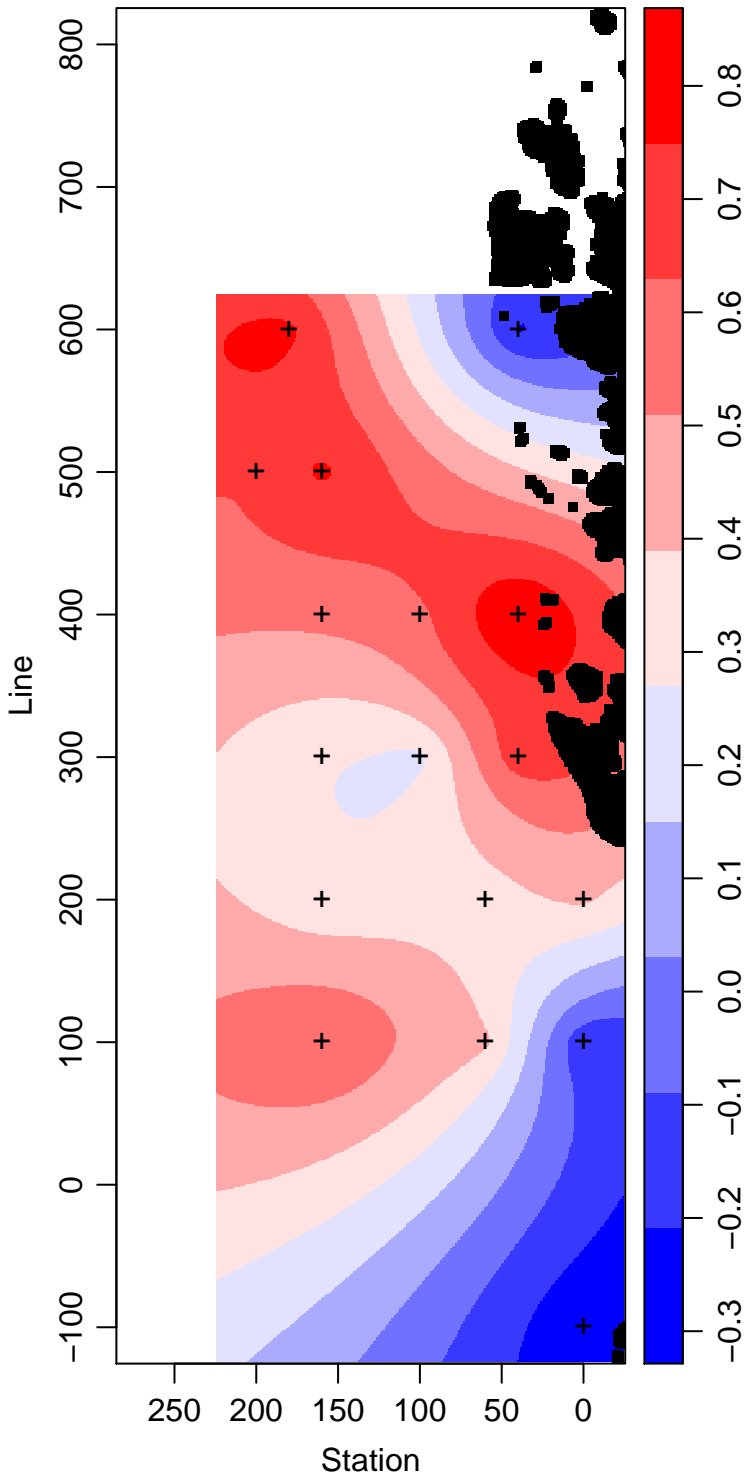
LMG09-01_35_Temperature ° Celsius
