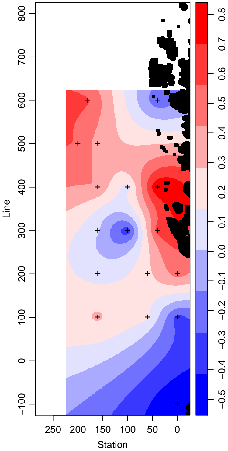
LMG09-01_45_Temperature ° Celsius
