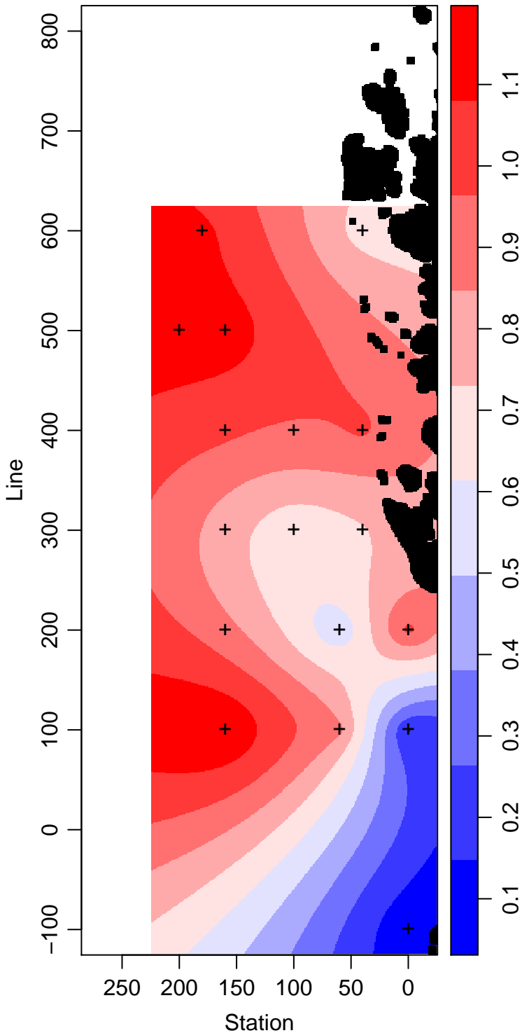
LMG09-01_5_Temperature ° Celsius
