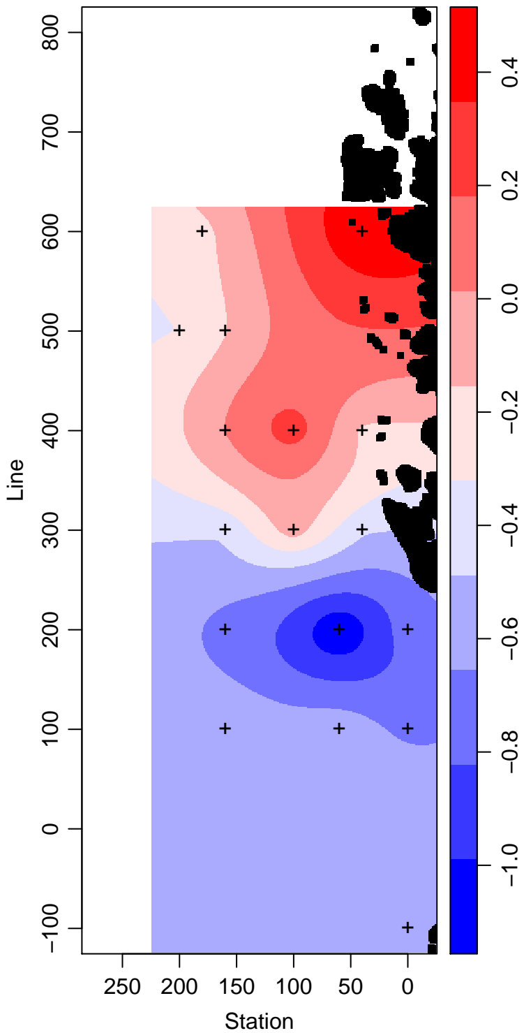
LMG09-01_90_Temperature ° Celsius
