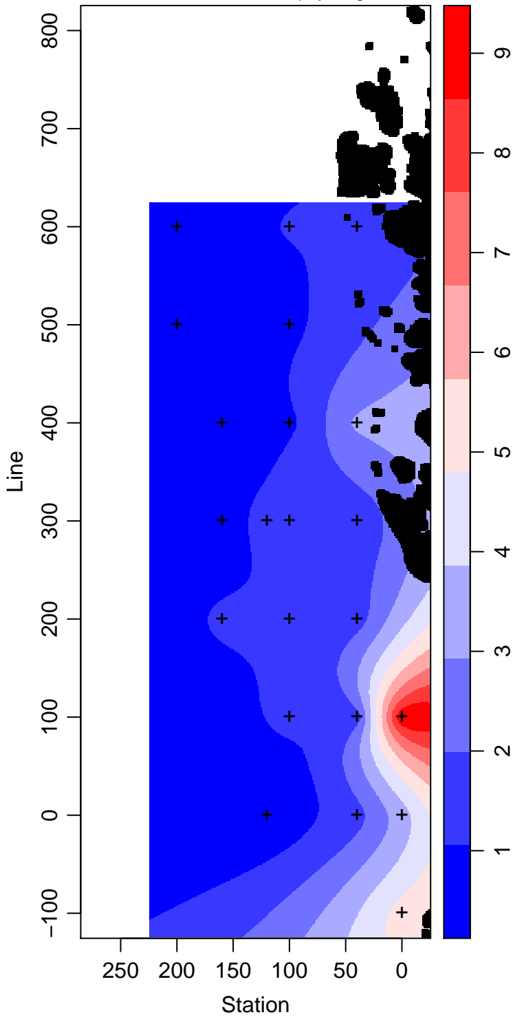
LMG10-01_20_Chlorophyll mg m -3
