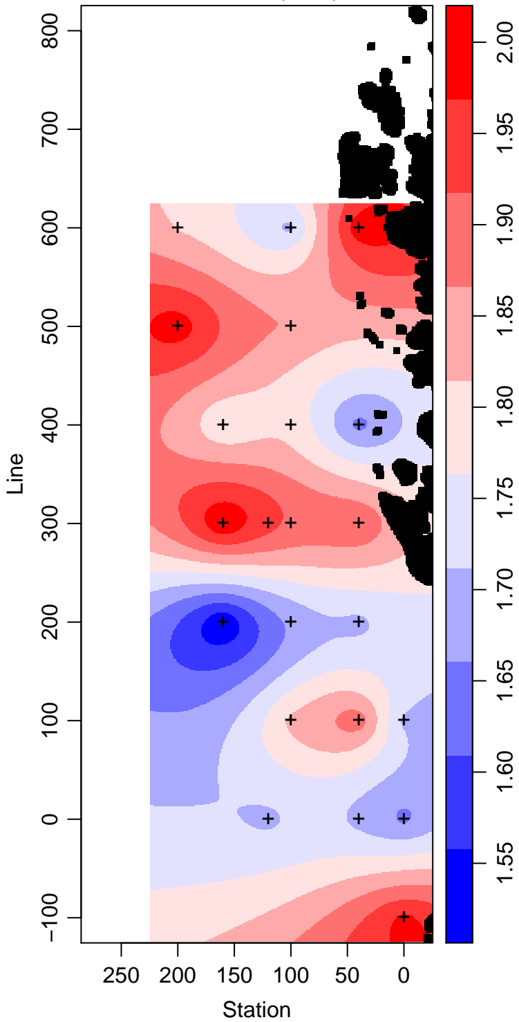
LMG10-01_60_Phosphate \mu\text{ mol L}^{-1}
