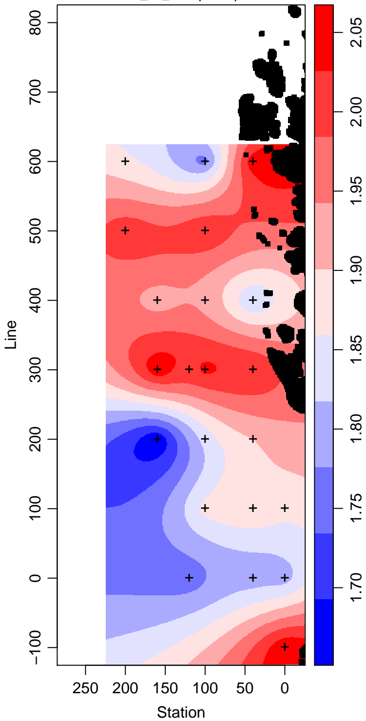
LMG10-01_70_Phosphate \mu\text{ mol L}^{-1}
