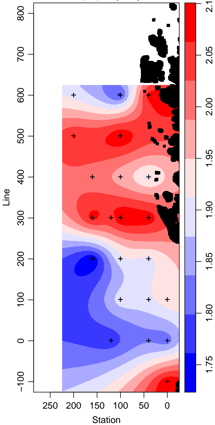
LMG10-01_75_Phosphate \mu\text{ mol L}^{-1}
