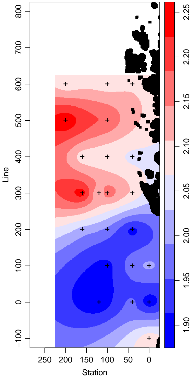
LMG10-01_95_Phosphate \mu\text{ mol L}^{-1}
