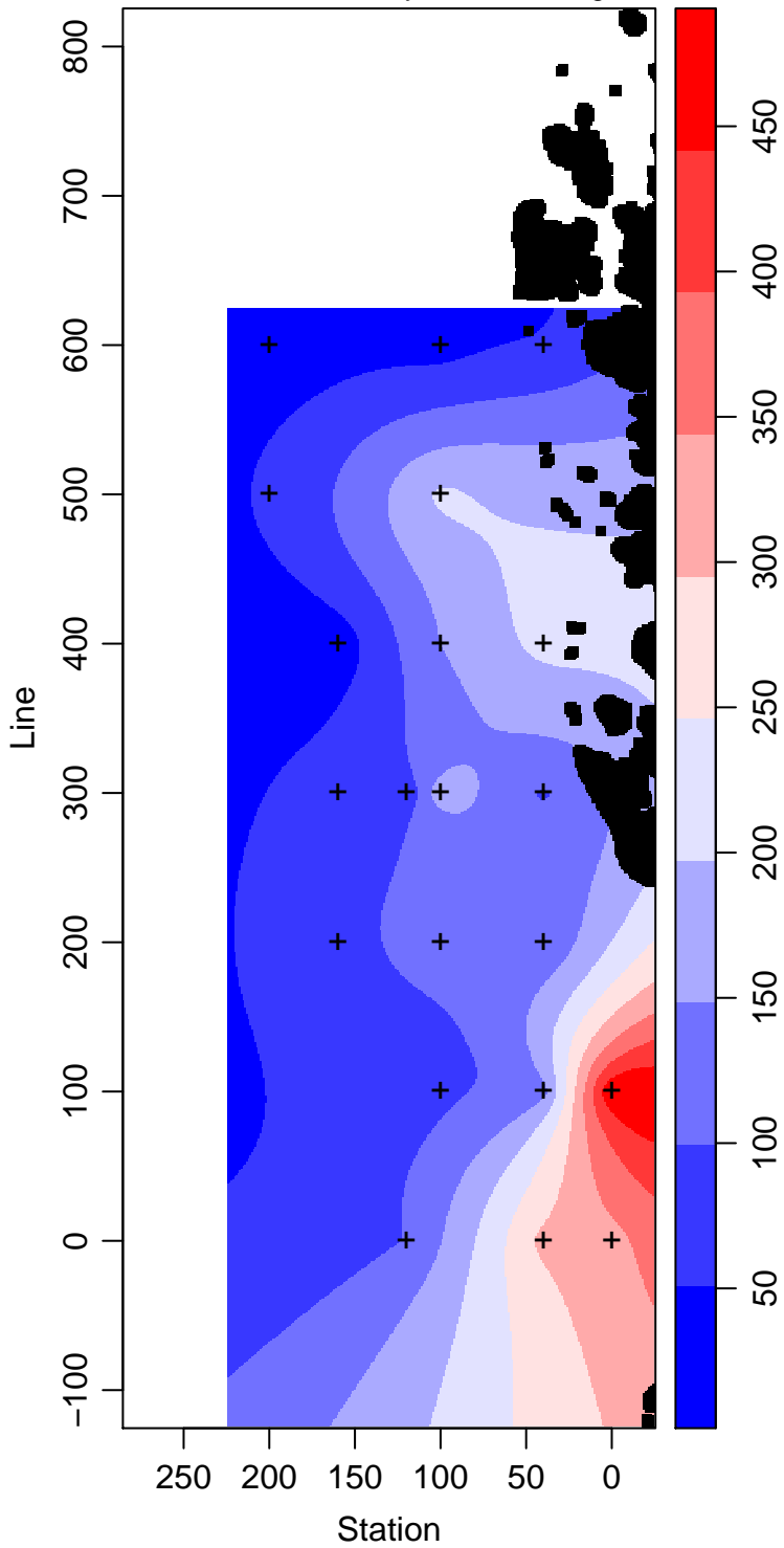
LMG10-01_20_Primary.Production mg m -3
