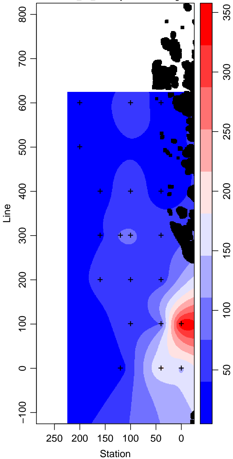
LMG10-01_50_Primary.Production mg m -3
