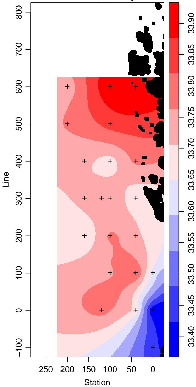
LMG10-01_30_Salinity
