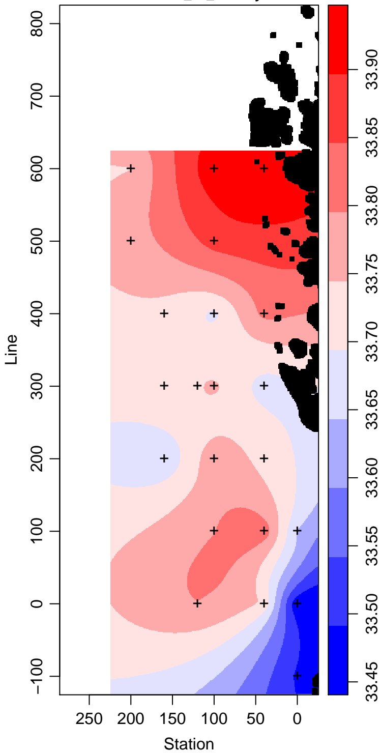
LMG10-01_40_Salinity
