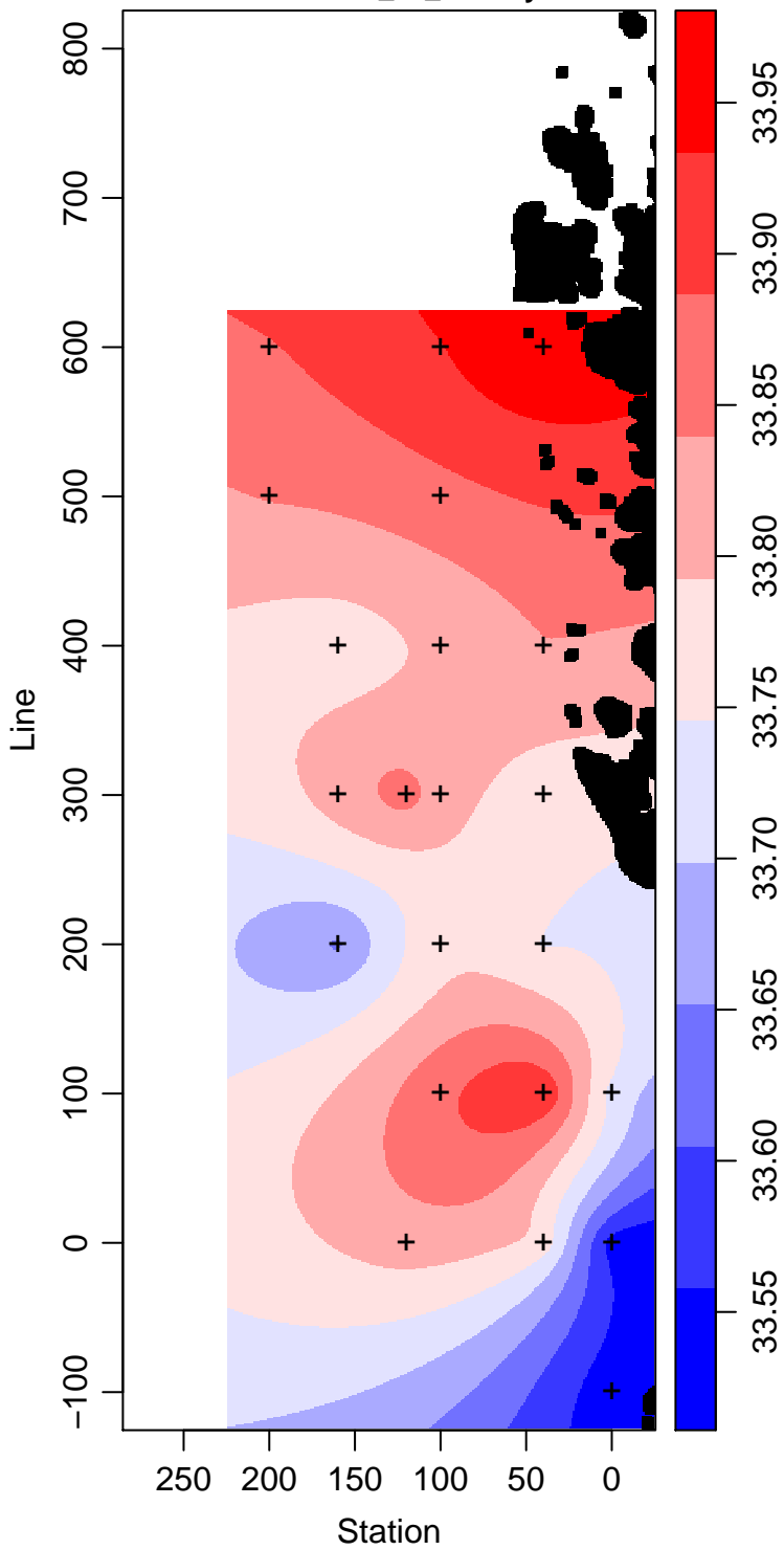
LMG10-01_50_Salinity
