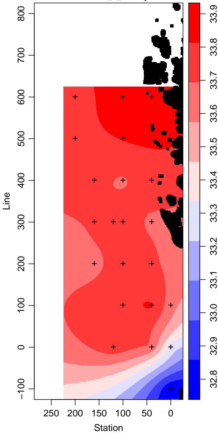
LMG10-01_5_Salinity
