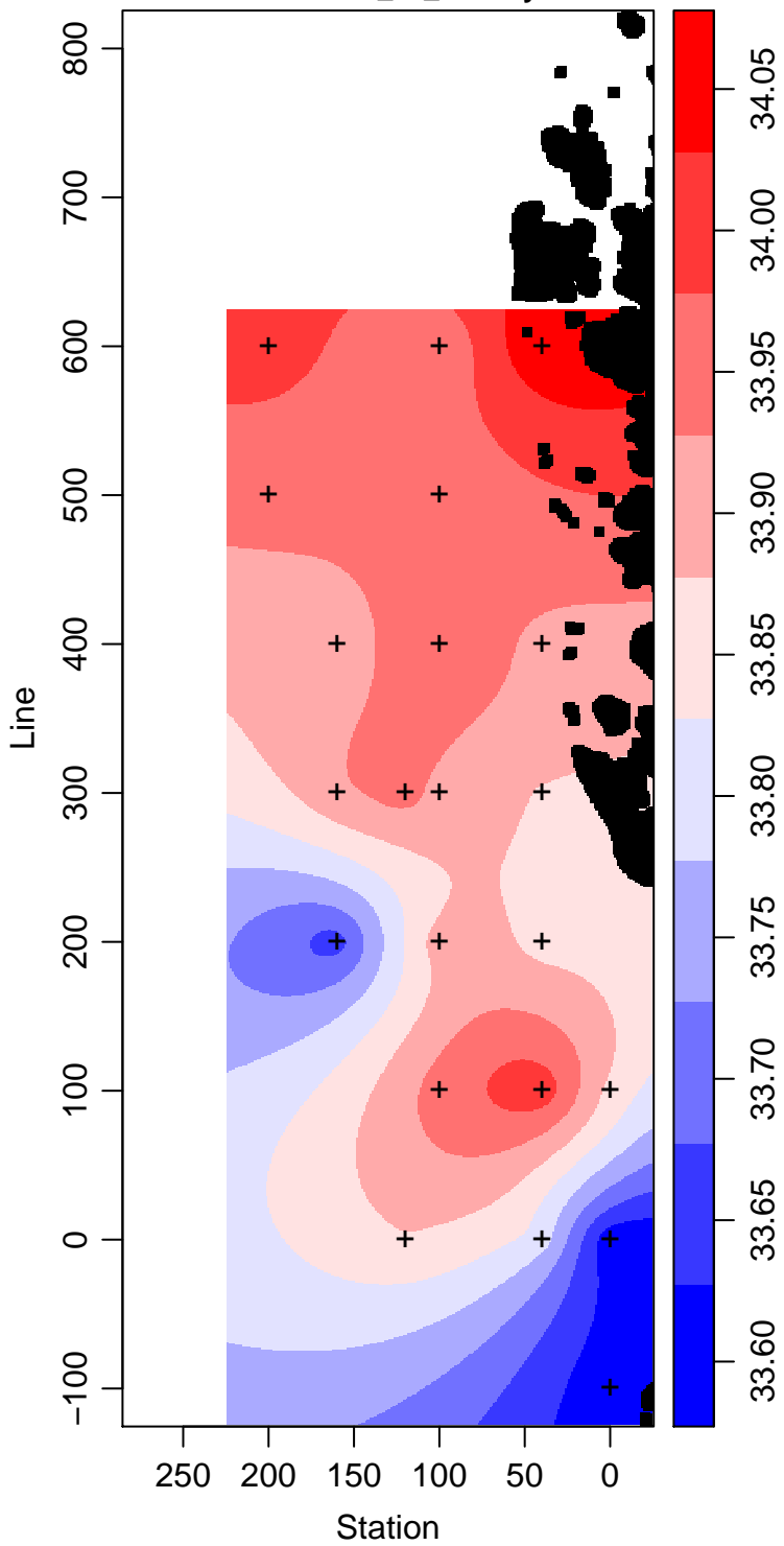
LMG10-01_60_Salinity
