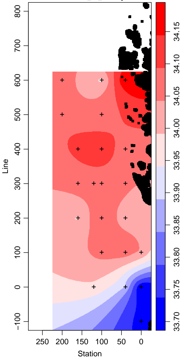
LMG10-01_80_Salinity
