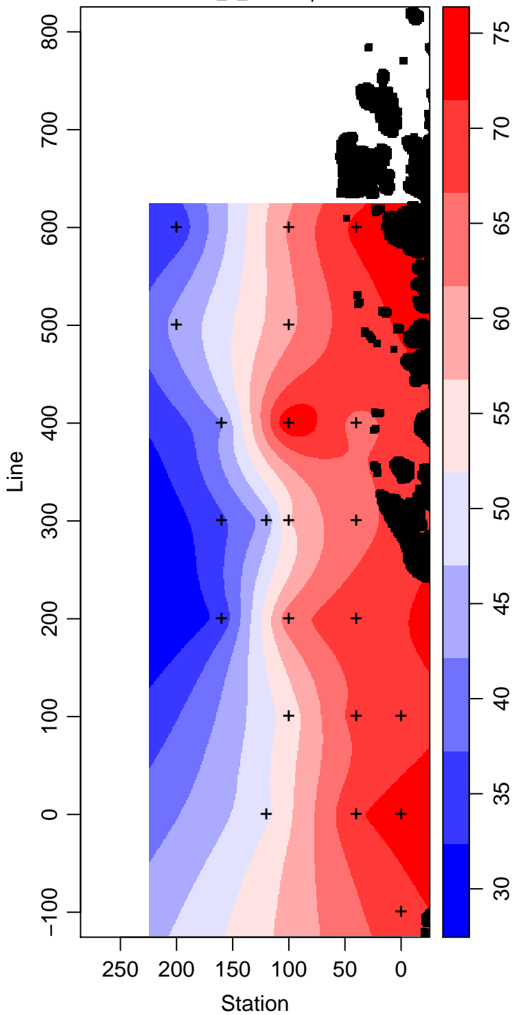
LMG10-01_1_Silicate \mu\text{ mol L}^{-1}
