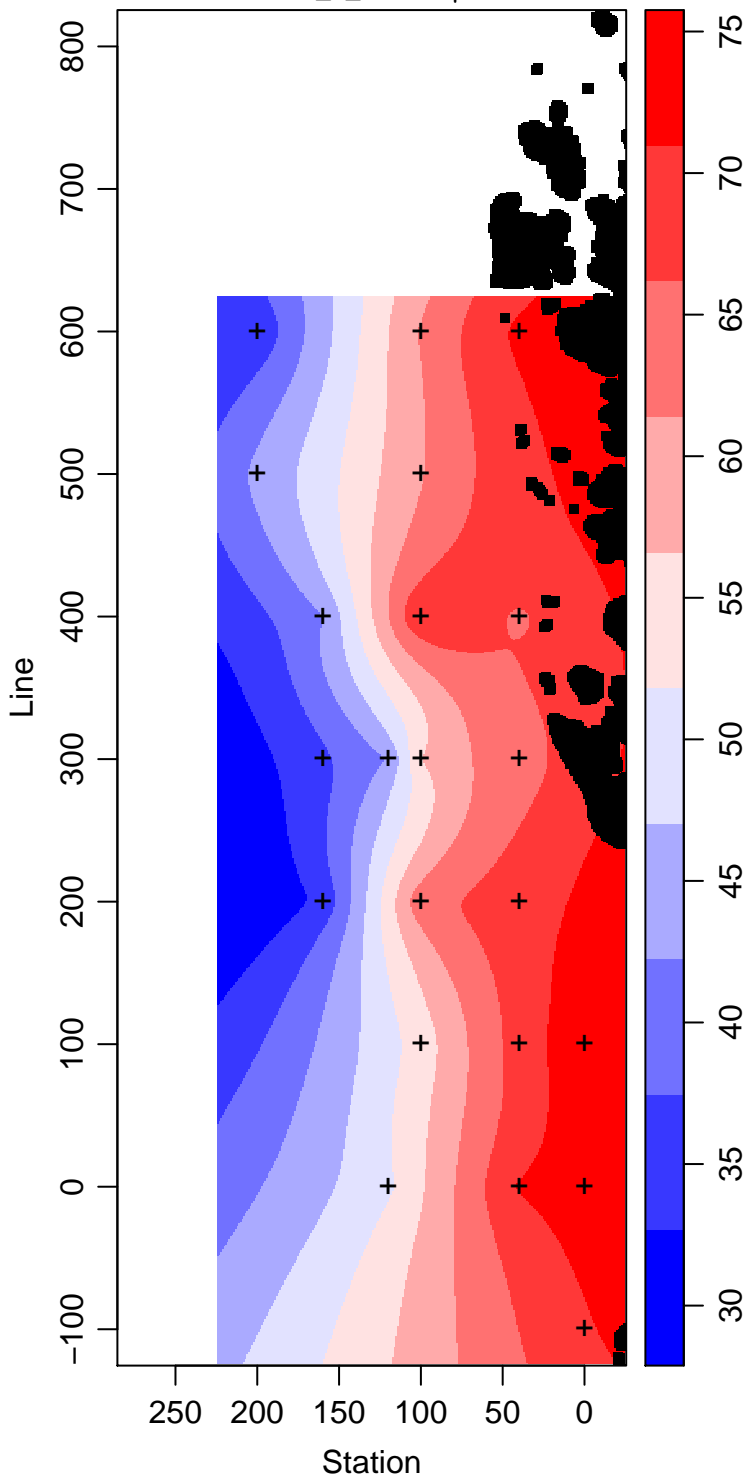
LMG10-01_5_Silicate \mu\text{ mol L}^{-1}
