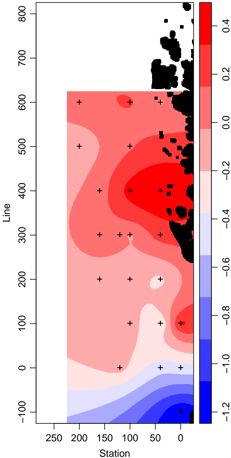
LMG10-01_40_Temperature ° Celsius
