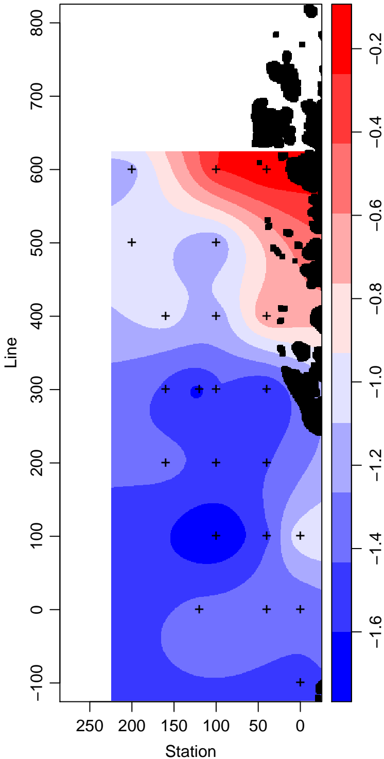
LMG10-01_85_Temperature ° Celsius
