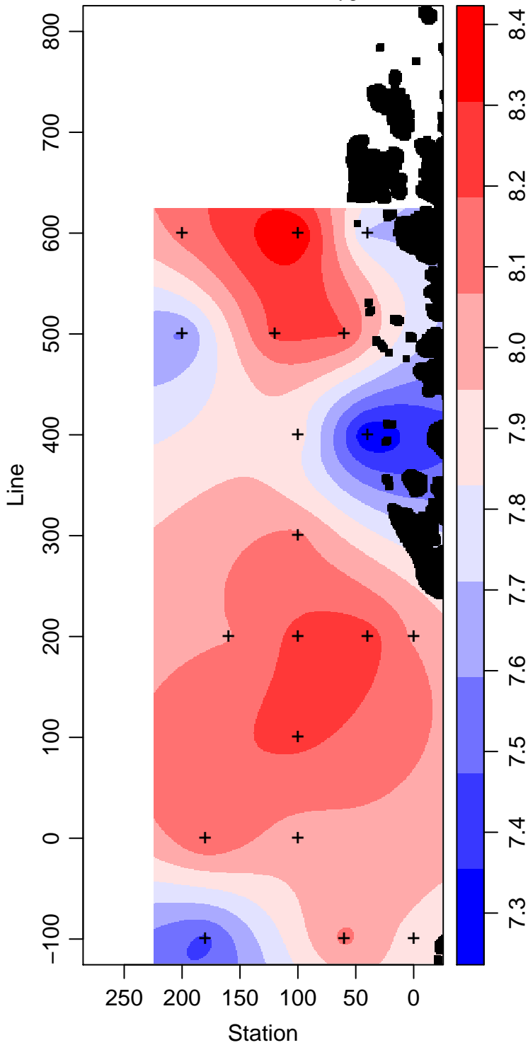
LMG11-01_65_Dissolved.Oxygen ml L -1
