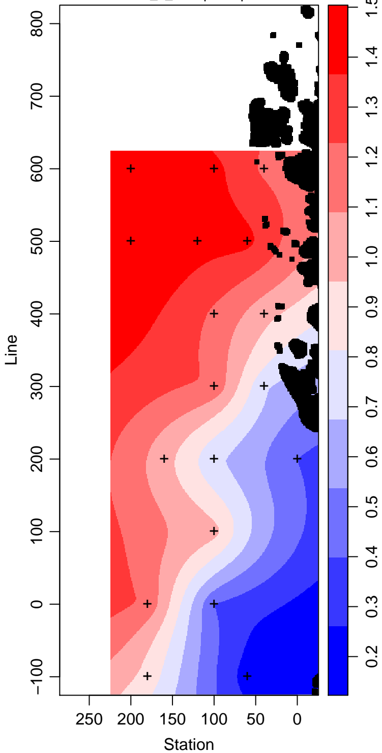
LMG11-01_1_Phosphate \mu\text{ mol L}^{-1}
