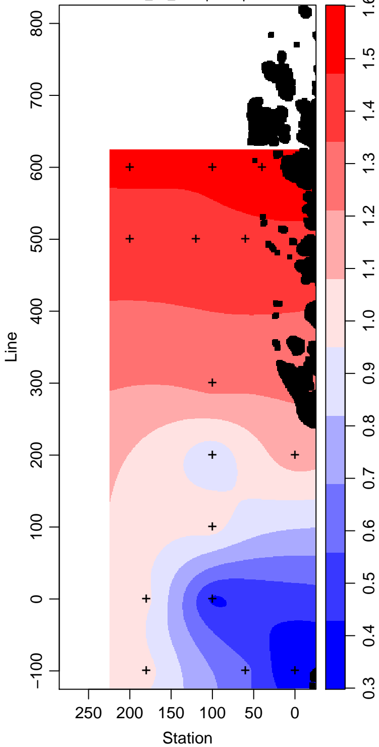
LMG11-01_25_Phosphate \mu\text{ mol L}^{-1}
