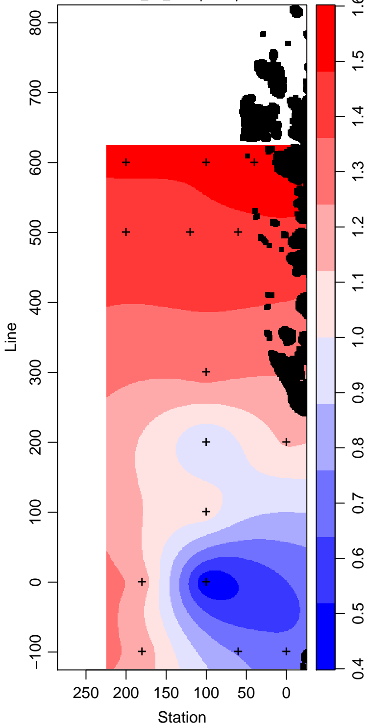
LMG11-01_30_Phosphate \mu\text{ mol L}^{-1}
