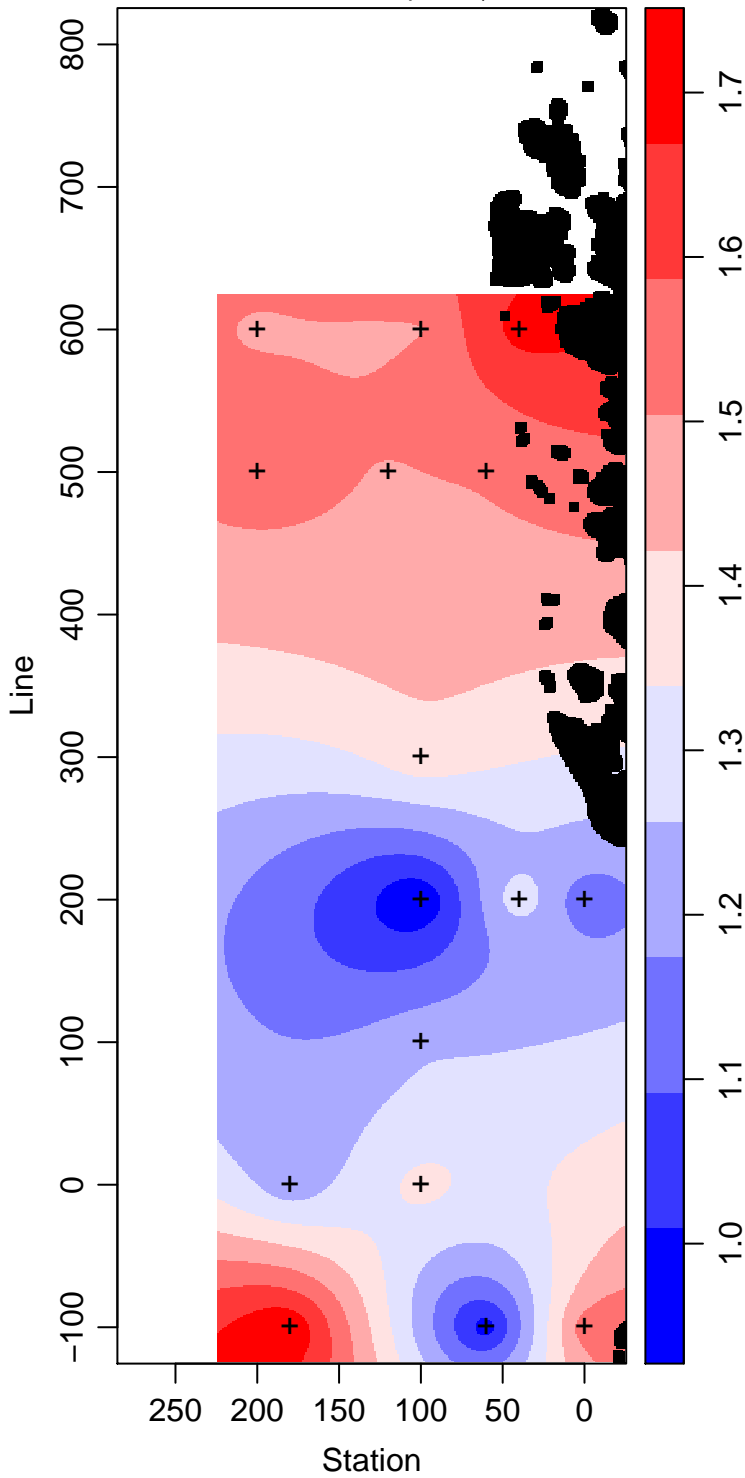
LMG11-01_45_Phosphate \mu\text{ mol L}^{-1}
