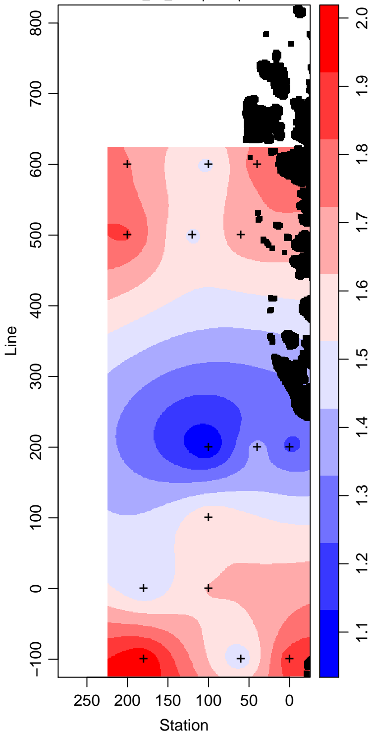
LMG11-01_75_Phosphate \mu\text{ mol L}^{-1}
