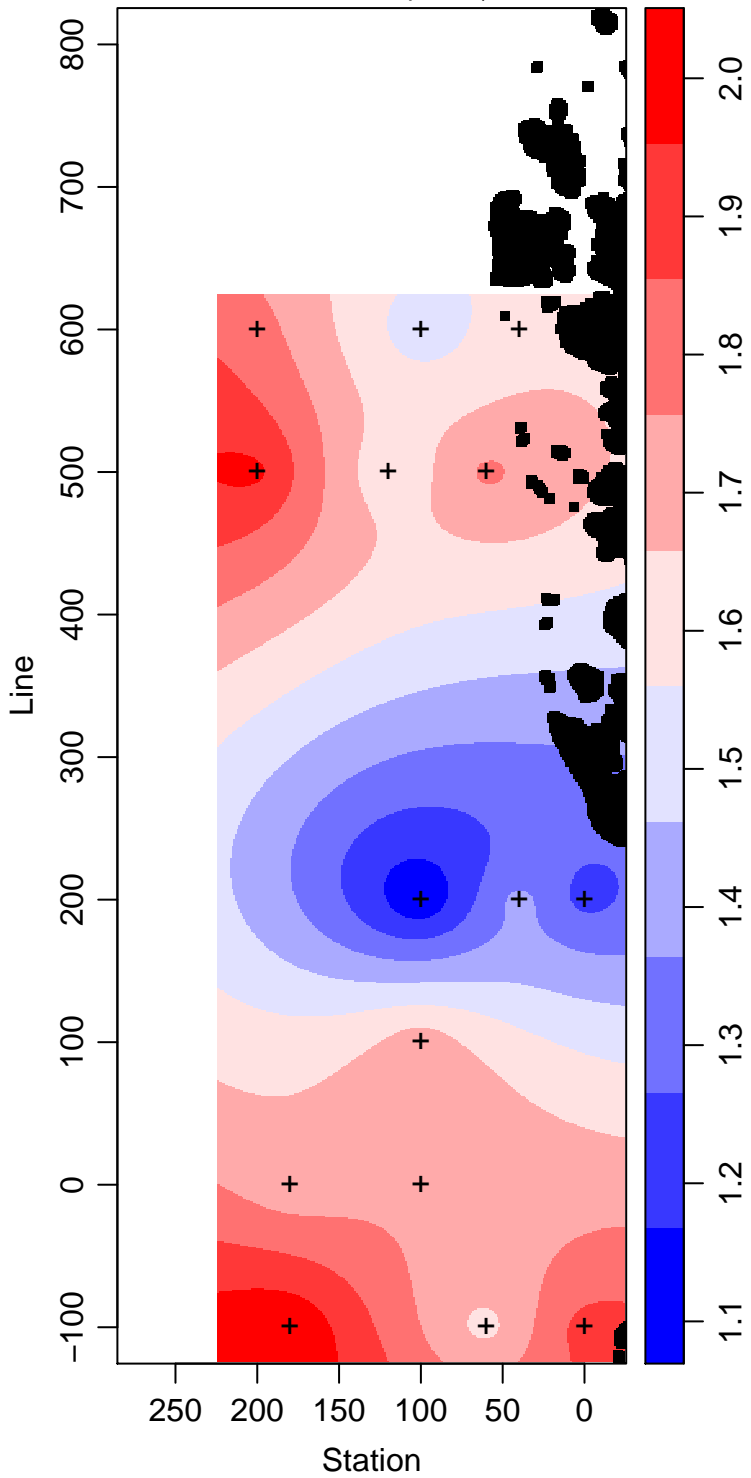
LMG11-01_85_Phosphate \mu\text{ mol L}^{-1}
