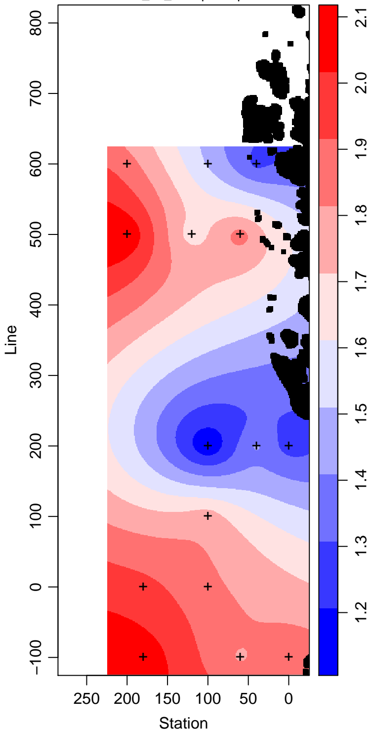
LMG11-01_95_Phosphate \mu\text{ mol L}^{-1}
