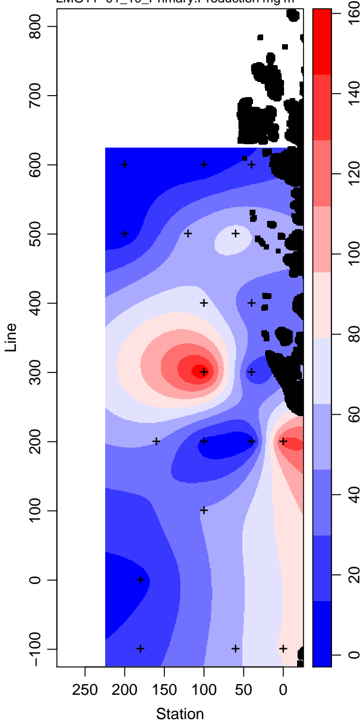
LMG11-01_10_Primary.Production mg m -3
