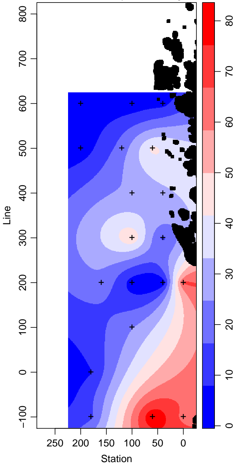
LMG11-01_20_Primary.Production mg m -3
