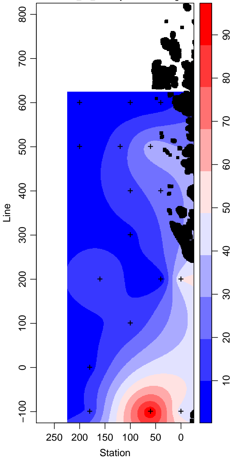
LMG11-01_25_Primary.Production mg m -3
