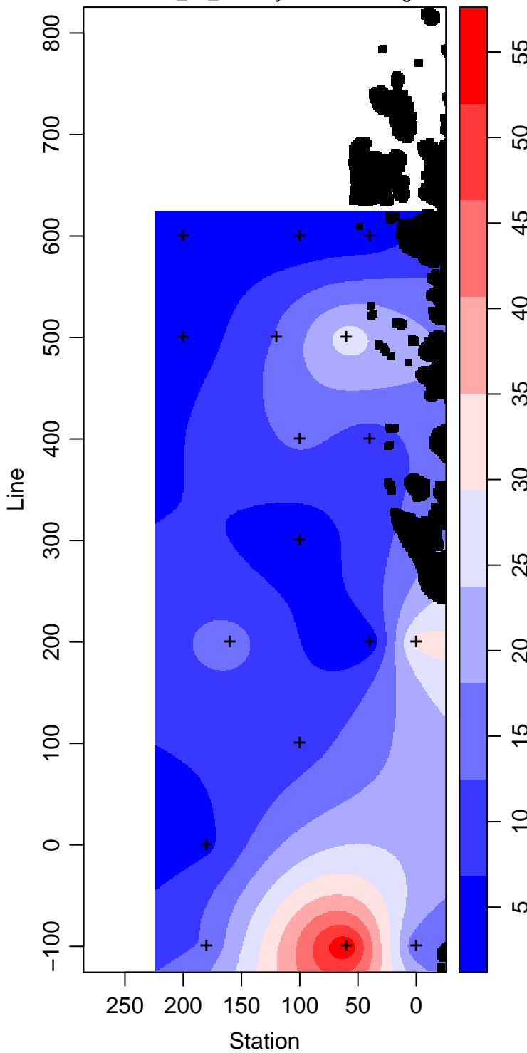
LMG11-01_30_Primary.Production mg m -3
