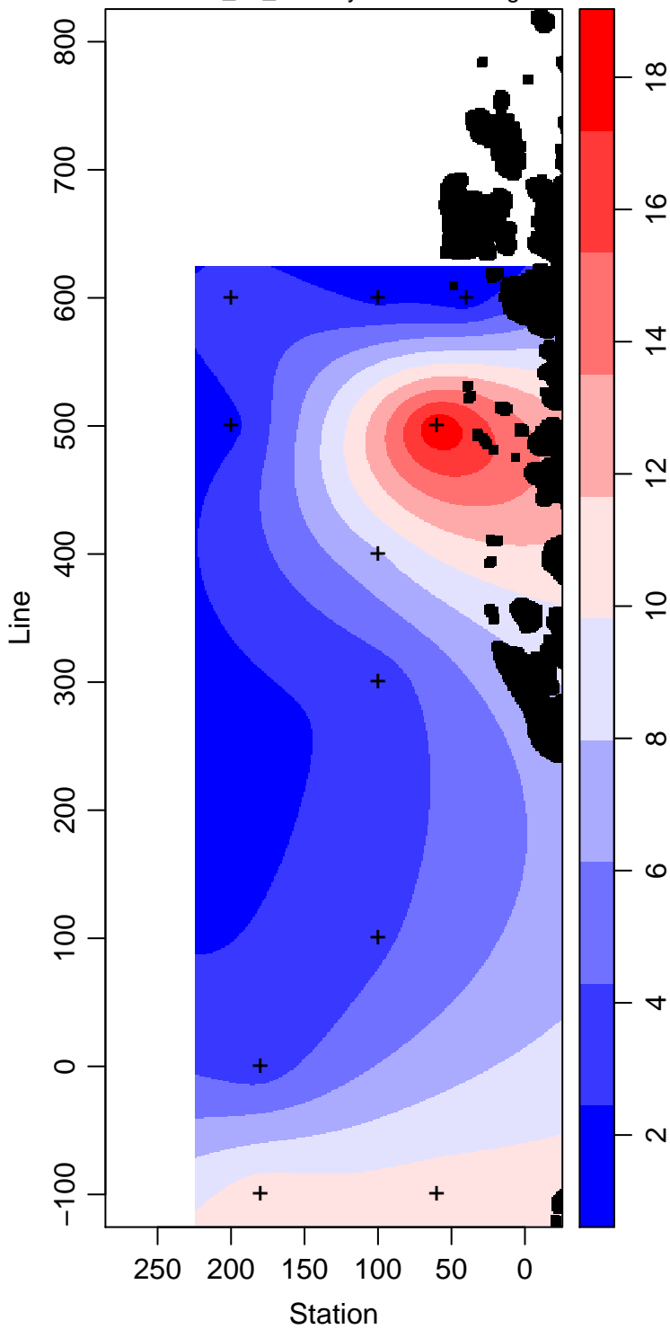
LMG11-01_45_Primary.Production mg m -3
