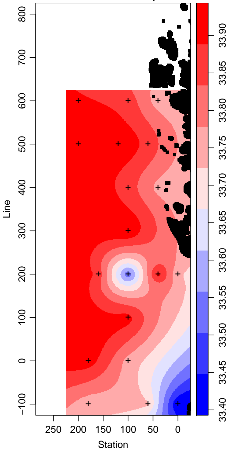
LMG11-01_30_Salinity
