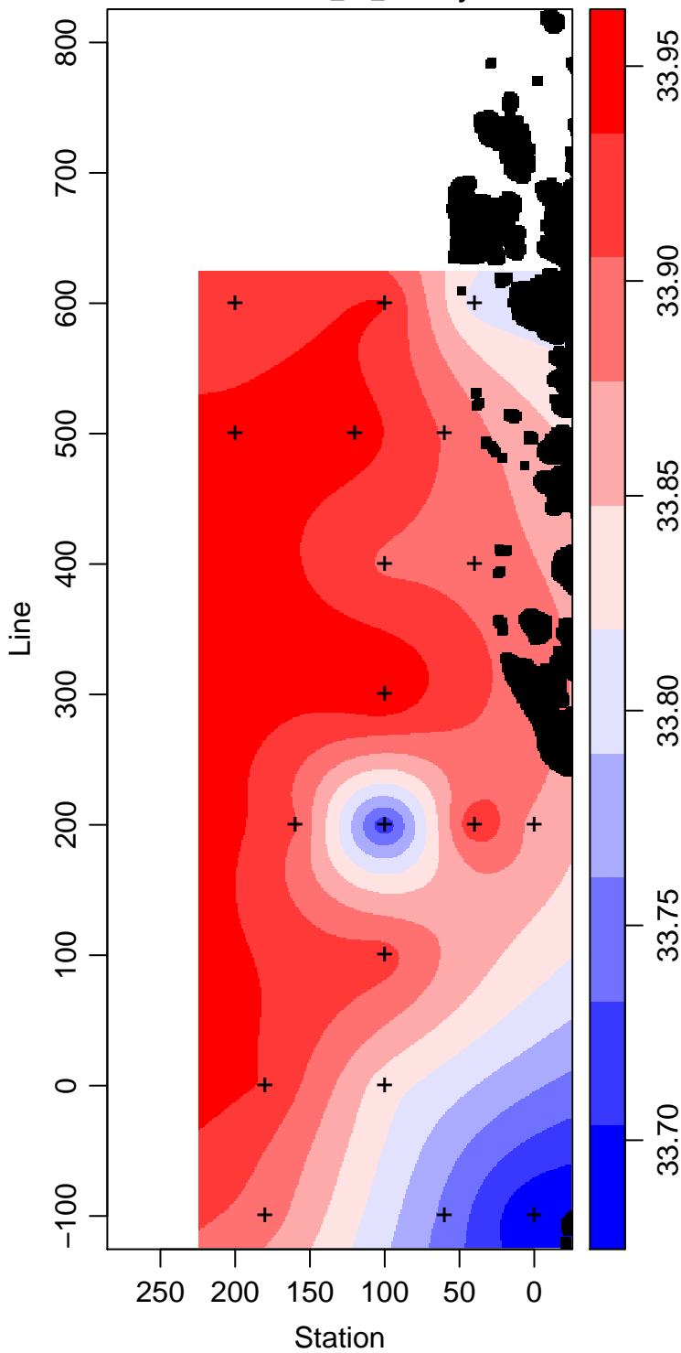
LMG11-01_50_Salinity
