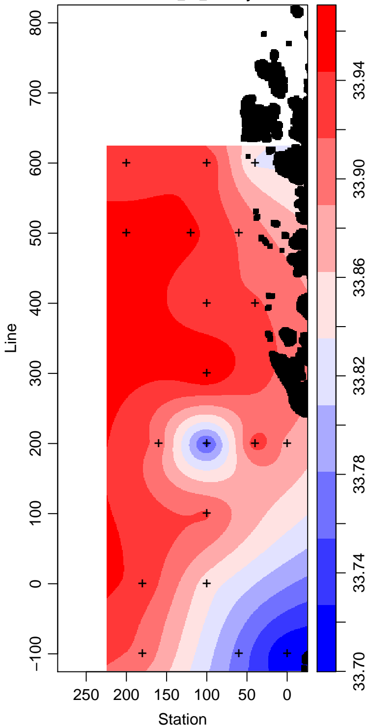
LMG11-01_55_Salinity
