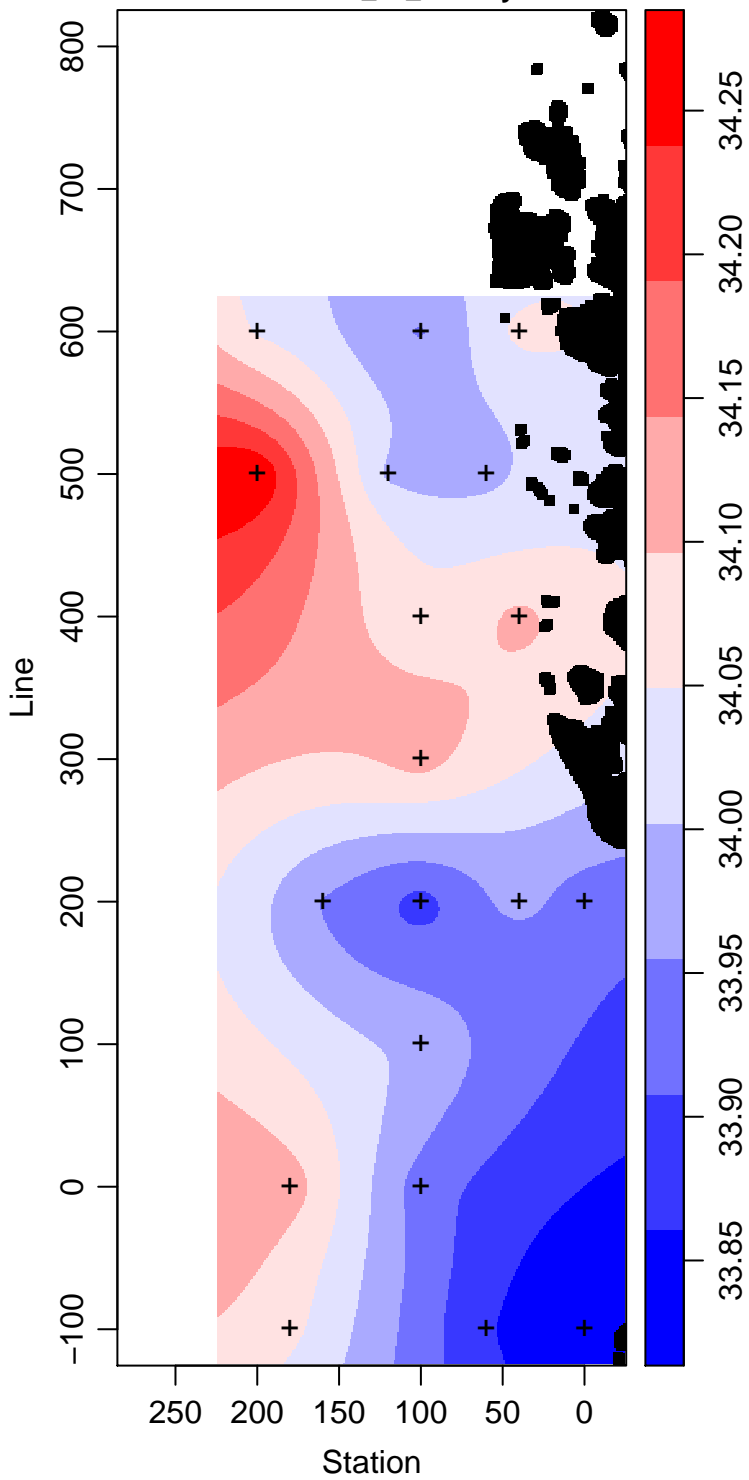
LMG11-01_90_Salinity
