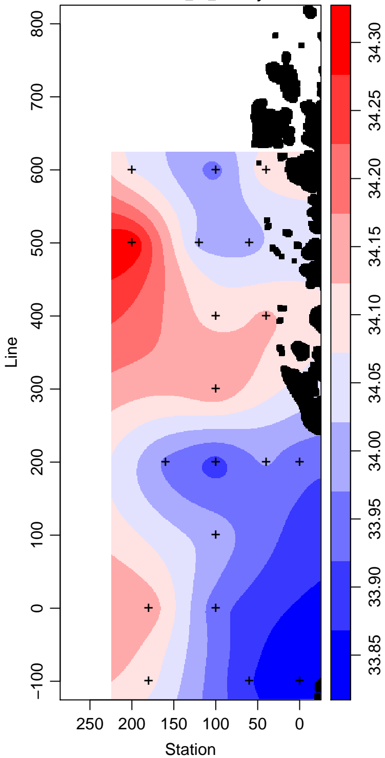
LMG11-01_95_Salinity
